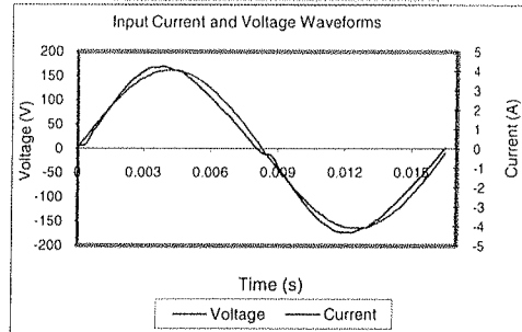
Input AC Current Waveform (THD = 10.55%, 50% Load)
